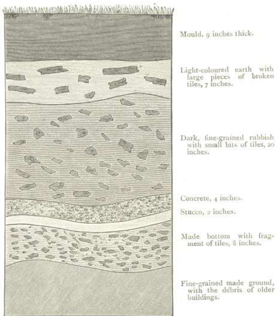
FIG. 12.—Section in the centre of the Basilica at Silchester.
