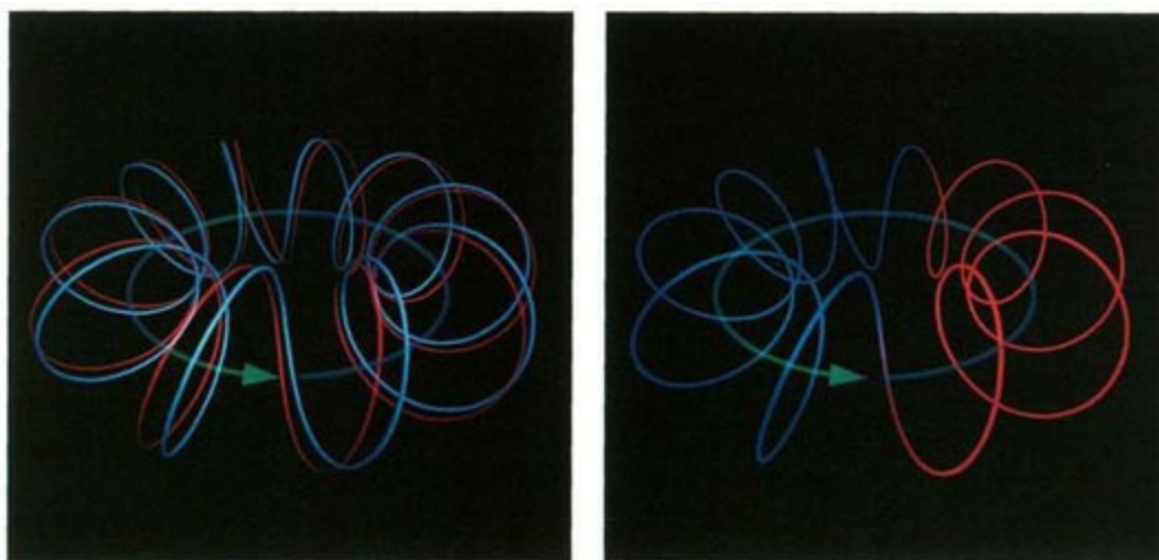
Waves in Atomic Orbits
